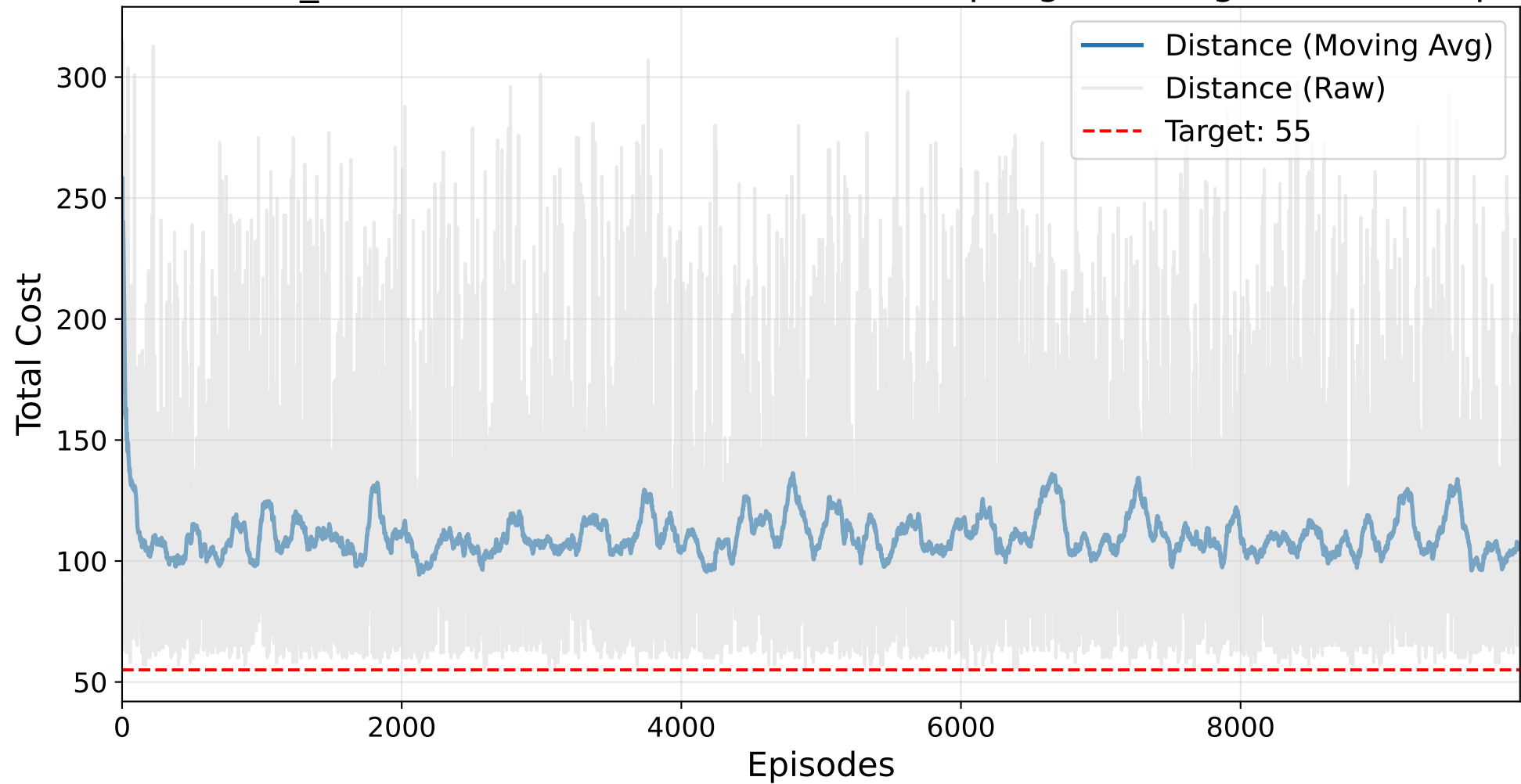
Final NO_MASK Masked AutoRL-SOP (Resampling) Training - br17.10.sop
